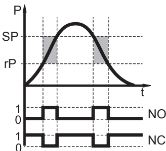
Windowed Mode
