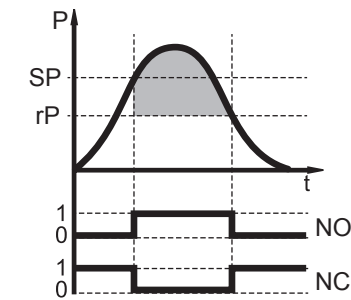
Hysteresis Mode
