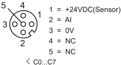
Input signal connection M12
