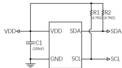
Recommended Application Circuit
